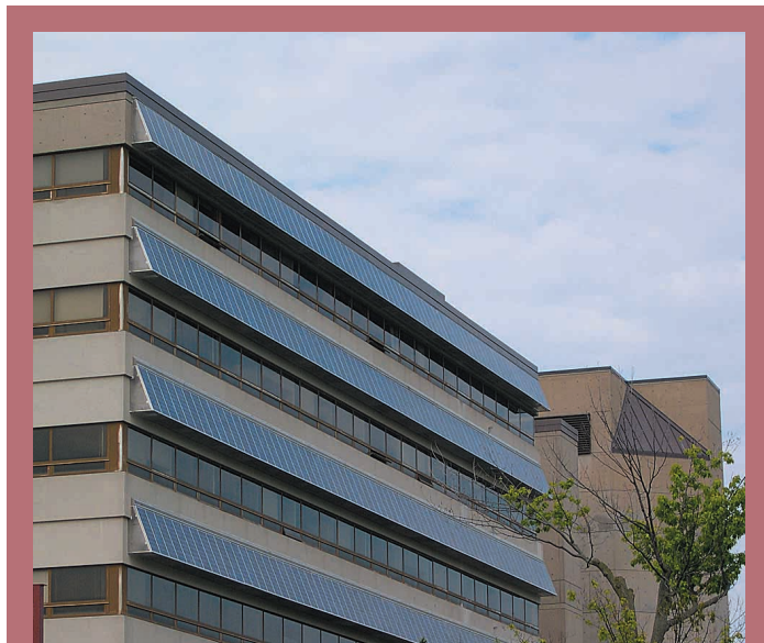
Figure 1: A 20 kW grid-connected, building-integrated PV system at Queen's University provides summer shading and year-round electricity. (Photo: Anton Driesse)
